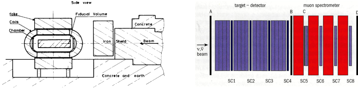
Figure 1 – Setup of the Gargamelle and E-1A (HPW) experiments
